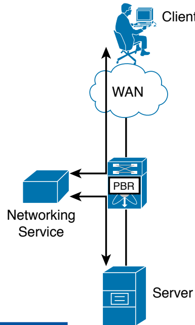
Policy-Based Router (PBR)
